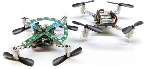
Figure 3: Bitcraze Crazyflie 2.0 with the rotors mounted upside down so they do not obscure the LEDs of the attached tracking marker and an unmodified platform for comparison in the background. With this modification, the motor mounts expose to the top and are used as interaction points.
