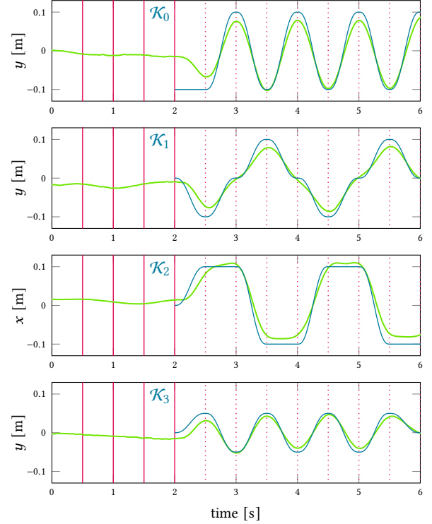
Figure 5: MetroDrone interaction sequences: Four taps to a beat at 120 bpm in 4/4 time signature (red), the propagated beat (dotted) to which a trajectory (blue) is initiated and a selected coordinate of the quadrotor's position (green) during flight of the trajectory.
